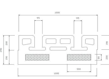
Floor slab S39
