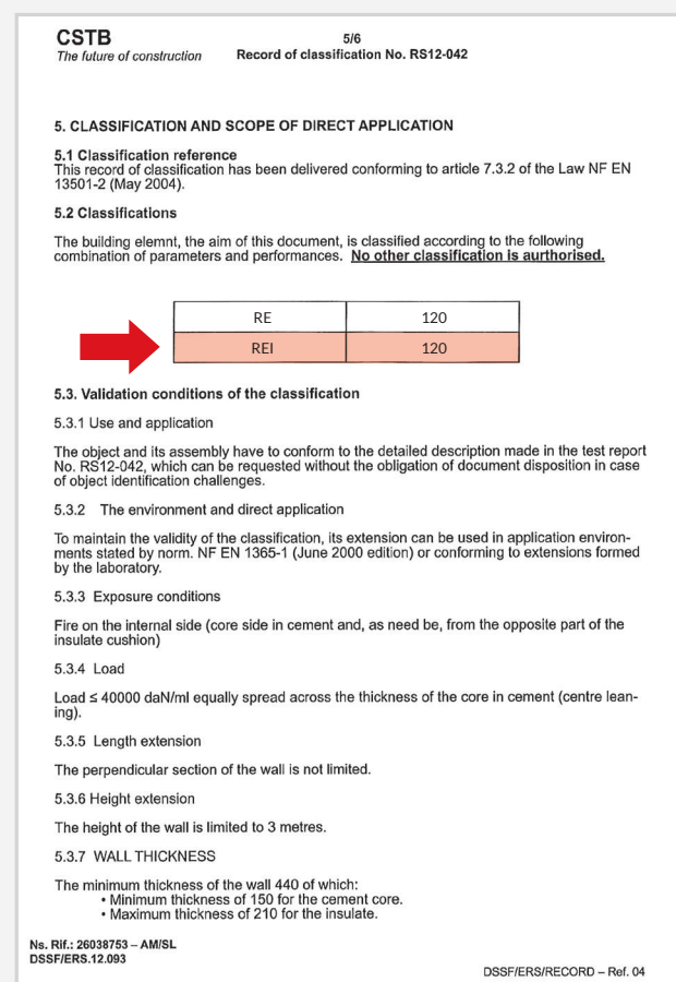
Certification of resistance to fire of plaster-less blocks
