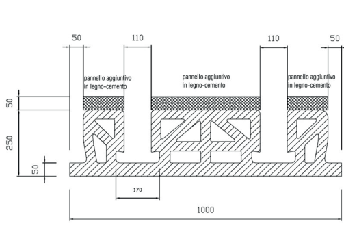
Floor slab S25+5
