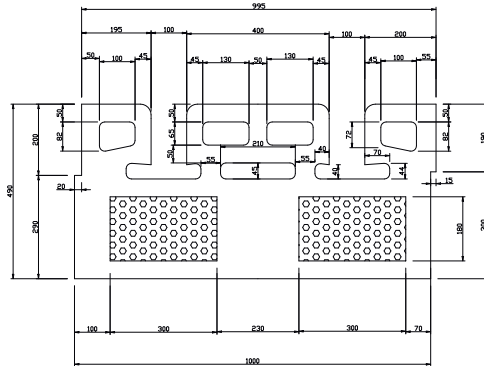
Floor slab S49
